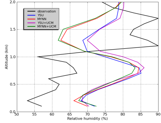
(b) RH on 24 May 2330 UTC at Trappes
