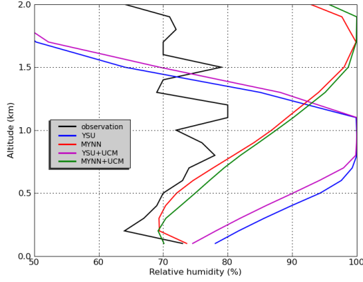
(a) RH on 23 May 2305 UTC at Trappes
