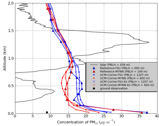
(a) PM_{10} on 24 May, 0357 UTC at Paris, Les Halles ( 48.86^\circ\text{N} , 2.35^\circ\text{E} )
