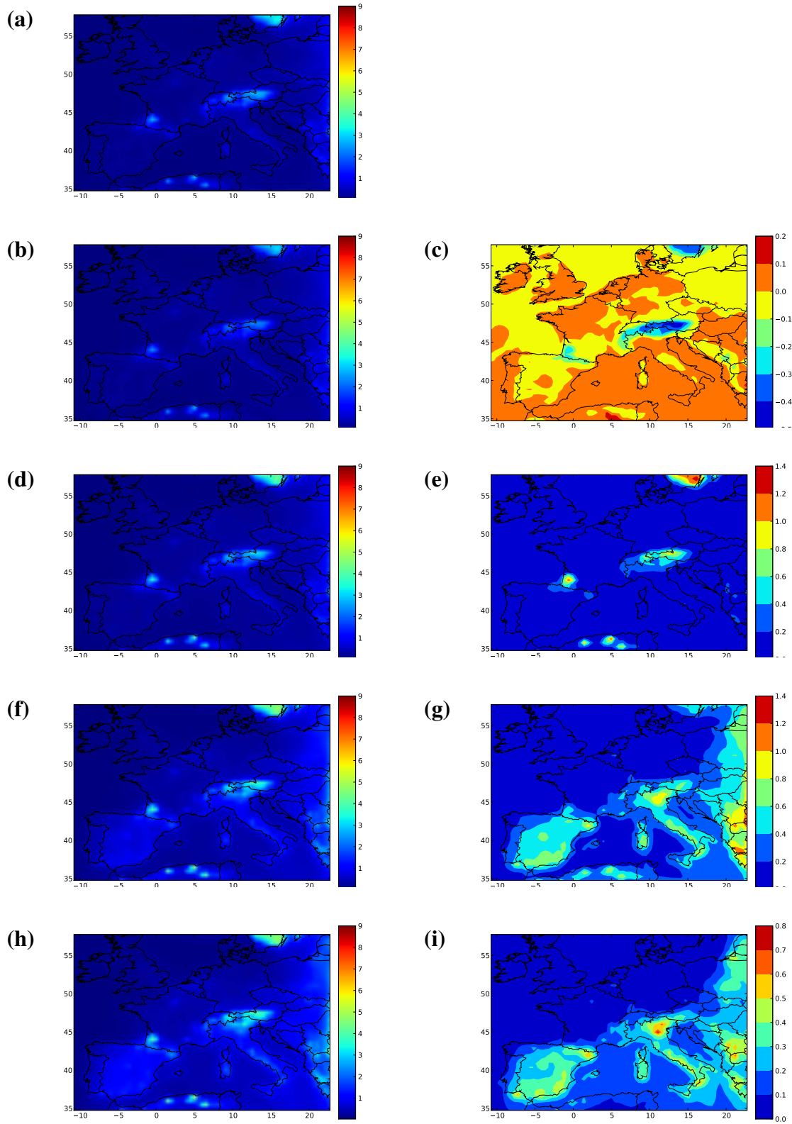
Figure 4.2: Simulations of PM 2.5 SOA (μg/m 3 ) over Europe with RACM2 for gas-phase chemistry and distinct SORGAM modules for SOA formation: (a) SORGAM (first row); (b) SORGAM- \Delta H (second row left); (c) [SORGAM- \Delta - SORGAM] (second row right); (d) SORGAM-NO x (third row left); (e) [SORGAM-NO x - SORGAM- \Delta H ] (third row right); (f) SORGAM-bio (fourth row left); (g) [SORGAM-bio - SORGAM-NO x ] (fourth row right); (h) Super-SORGAM (fifth row left); (i) [Super-SORGAM - SORGAM-bio] (fifth row right).
