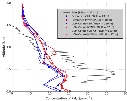
(c) PM_{10} on 25 May, 0309 UTC at Palaiseau ( 48.71^\circ\text{N} , 2.22^\circ\text{E} )
