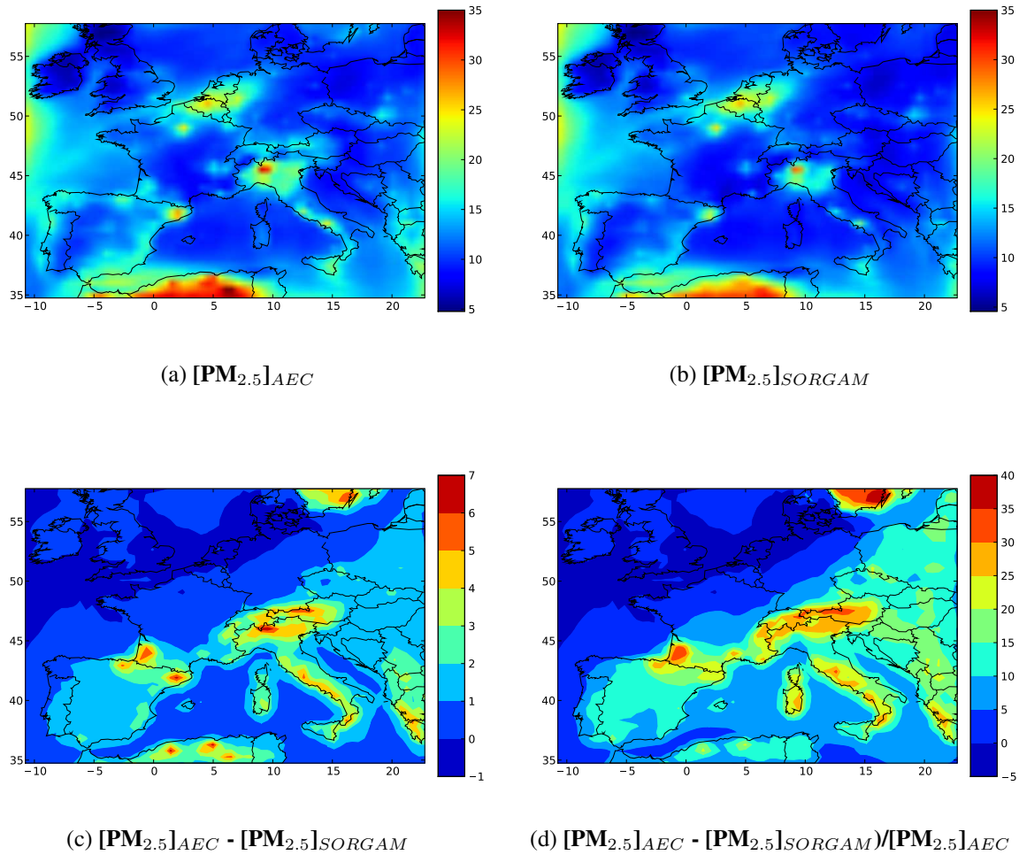
Figure 4.1: PM 2.5 concentrations ( \mu\text{g}/\text{m}^3 ) over Europe simulated with AEC and SORGAM for SOA formation and RACM2 for gas-phase chemistry. Results are averaged over the 1-month simulation of 15 July to 15 August 2001: (a) [\text{PM}_{2.5}]_{\text{AEC}} (top left); (b) [\text{PM}_{2.5}]_{\text{SORGAM}} (top right); (c) [\text{PM}_{2.5}]_{\text{AEC}} - [\text{PM}_{2.5}]_{\text{SORGAM}} (bottom left); (d) ([\text{PM}_{2.5}]_{\text{AEC}} - [\text{PM}_{2.5}]_{\text{SORGAM}})/[\text{PM}_{2.5}]_{\text{AEC}} (bottom right)
