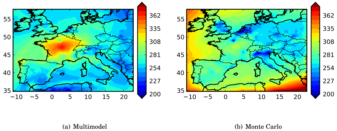
Figure 4.6: Ozone spatial covariance fields for the multimodel sub-ensemble and the Monte Carlo sub-ensemble, in \mu\text{g}^2\text{m}^{-6} . The location with respect to which the covariance is computed is a background cell in the center of France.
