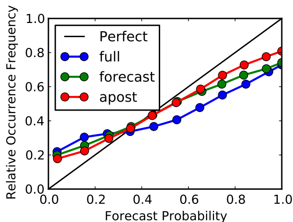
(a) \text{NO}_2 \geq 50 \mu\text{g m}^{-3}
