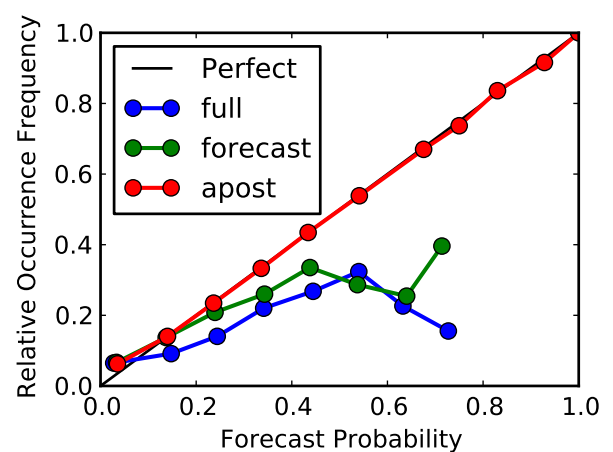
(b) \text{NO}_2 \geq 100 \mu\text{g m}^{-3}
